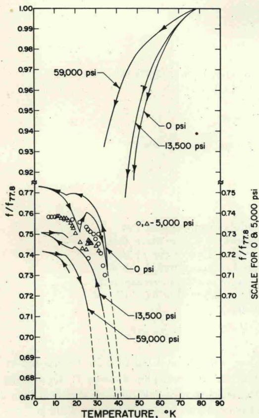
FIG. 1. Effects of pressure on the basic data for C_{11} vs. temperature. ( C_{11} = \rho V_{[100]}^2 , \rho = density).
